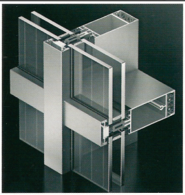
Schuco FW50+-SI Curtain Wall System (Image Provided by Schuco USA)
